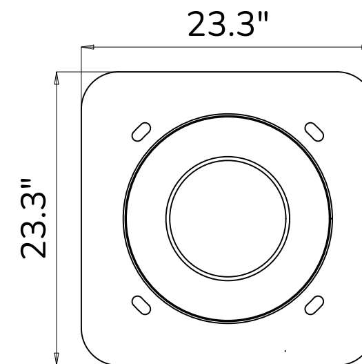
16" Top Adapter (2476842000)
